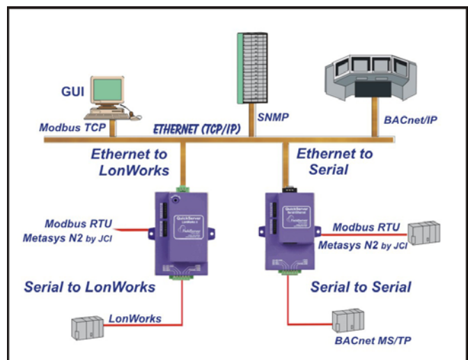
LonWorks FS-QS-1011-XXXX
